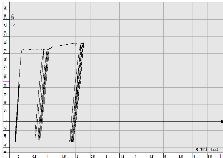
Tension & compression cyclic test
